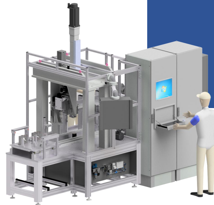
Joining machine with downstream pull-off test
